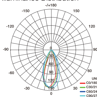
Illuminance Distribution
