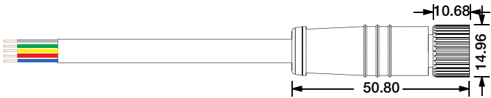
Female Connector M12-F-5C-20AWG-D6-W-0327-S
