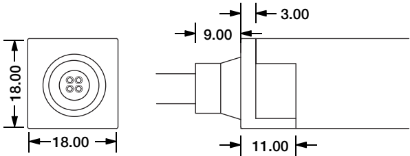
Direct Entry Connector MJ-SFW20-RGB-D01/02/03 MJ-SFW20-RGB-D01SM MJ-SFW20-RGB-D02SF MJ-SFW20-RGB-D03SFM
