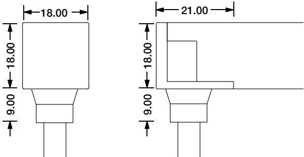
Bottom Entry Connector MJ-SFW20-RGB-B01/02/03 MJ-SFW20-RGB-B01SM MJ-SFW20-RGB-B02SF MJ-SFW20-RGB-B03SFM
