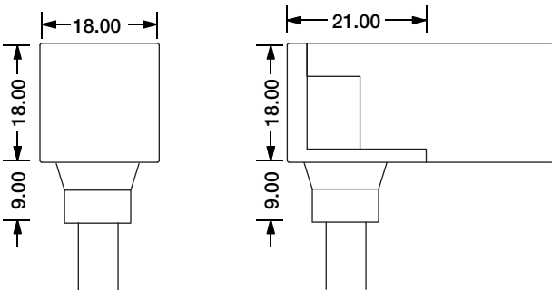
Bottom Entry Connector MJ-SFW20-D3-B02SM MJ-SFW20-D3-B03SFM
