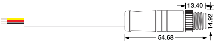
Male Connector M12-M-3C-20AWG-D6-W-0327-S
