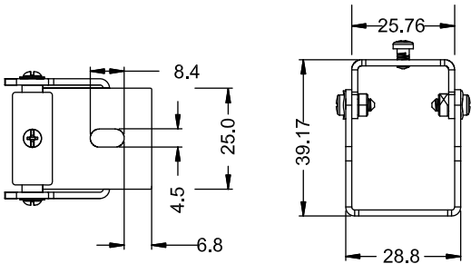
Angle Adjustable Bracket SFW20-ACC-HX-S2830C2
