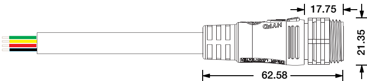
Male Connector SQ19-M-4C-20AWG-D8-W-0327-S
