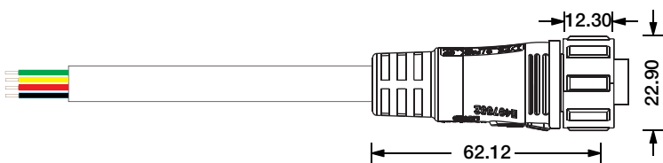
Female Connector SQ19-F-4C-20AWG-D8-W-0327-S
