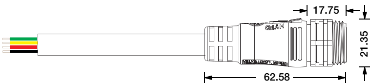
Male Connector SQ19-M-4C-20AWG-D8-W-0327-S
