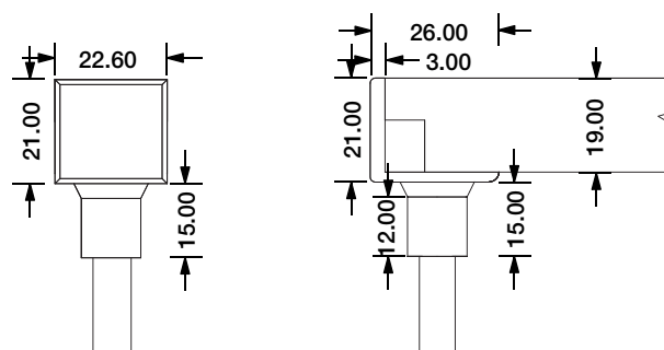
Bottom Entry Connector MJ-SF34-D3-B02SM MJ-SF34-D3-B03SFM
