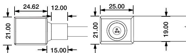
Side Entry Connector MJ-SF34-D3-S02SM MJ-SF34-D3-S03SFM
