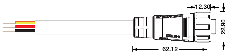
Female Connector SQ19-F-3C-20AWG-D8-0327-S
