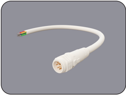
Male Connector SQ19-M-5C-15AWG+24AWG-D8-W-0327-S
