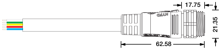
Male Connector SQ19-M-5C-15AWG+24AWG-D8-W-0327-S
