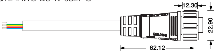
Female Connector SQ19-F-5C-15AWG+24AWG-D8-W-0327-S
