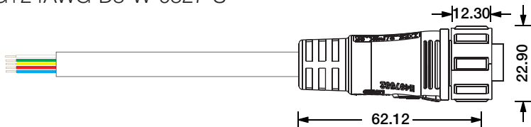
Female Connector SQ19-F-5C-18AWG+24AWG-D8-W-0327-S
