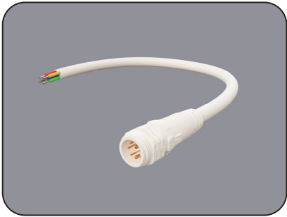
Male Connector SQ19-M-5C-18AWG+24AWG-D8-W-0327-S
