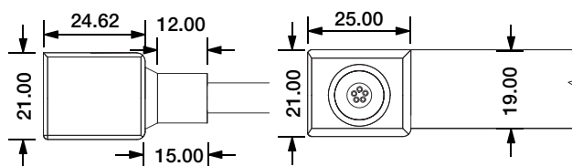
Side Entry Connector MJ-SF34-D5-S02SM MJ-SF34-D5-S03SFM
