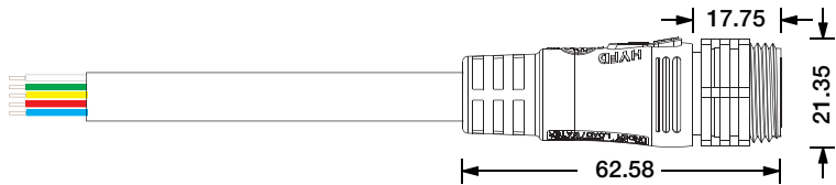
Male Connector SQ19-M-5C-18AWG+24AWG-D8-W-0327-S
