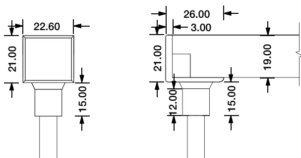
Bottom Entry Connector MJ-SF34-D5-B02SM MJ-SF34-D5-B03SFM
