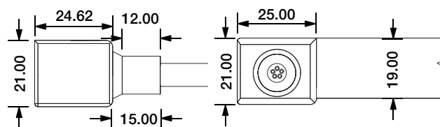
Side Entry Connector MJ-SF34-D5-S02SM MJ-SF34-D5-S03SFM
