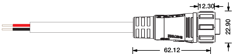
Female Connector SQ19-F-2C-15AWG-D8-0327
