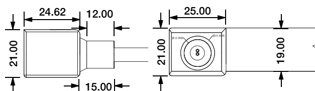
Side Entry Connector MJ-SF34-A-S01/02/03 MJ-SF34-A-S01SM MJ-SF34-A-S02SF MJ-SF34-A-S03SFM
