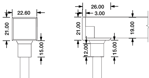
Bottom Entry Connector MJ-SF34-A-B01/02/03 MJ-SF34-A-B01SM MJ-SF34-A-B02SF MJ-SF34-A-B03SFM
