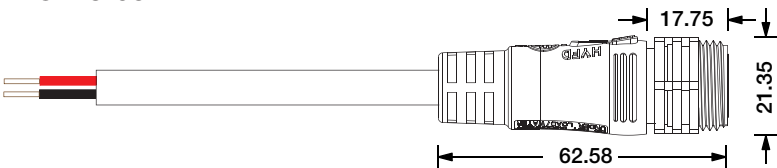
Male Connector SQ19-M-2C-15AWG-D8-0327
