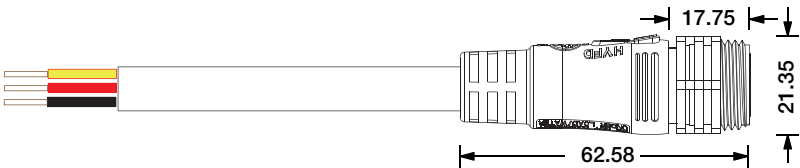
Male Connector SQ19-M-3C-20AWG-D8-0327-S
