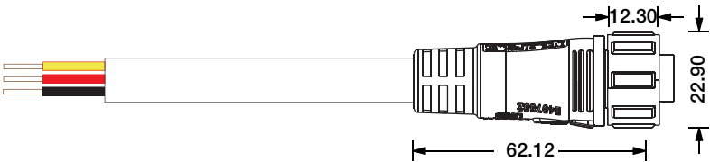
Female Connector SQ19-F-3C-20AWG-D8-0327-S
