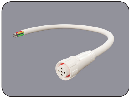
Female Connector SQ19-F-5C-20AWG-D8-W-0327-S
