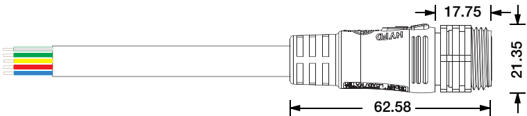
Male Connector SQ19-M-5C-20AWG-D8-W-0327-S
