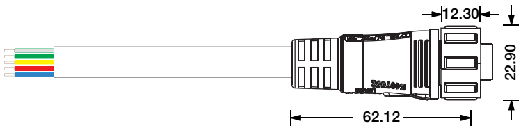
Female Connector SQ19-F-5C-20AWG-D8-W-0327-S
