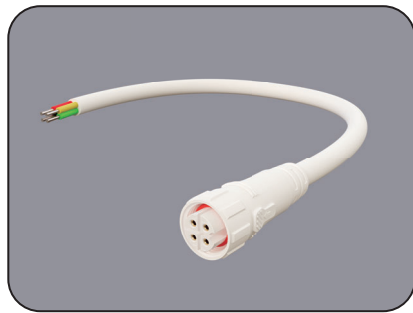
Female Connector SQ19-F-4C-20AWG-D8-W-0327-S
