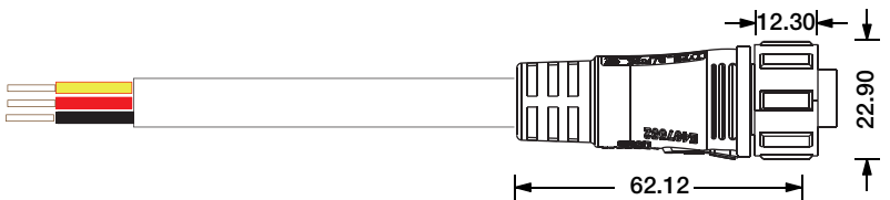
Female Connector SQ19-F-3C-20AWG-D8-0327-S
