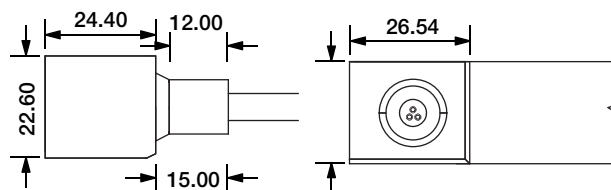
Side Entry Connector MJ-SF33-D3-S02SM MJ-SF33-D3-S03SFM
