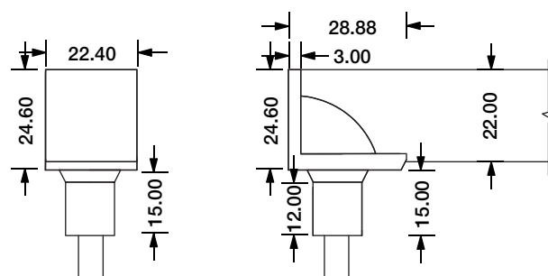
Bottom Entry Connector MJ-SF33-D3-B02SM MJ-SF33-D3-B03SFM
