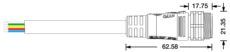
Male Connector SQ19-M-5C-18AWG+24AWG-D8-W-0327-S
