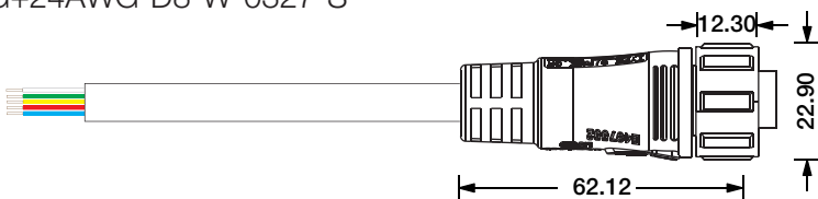
Female Connector SQ19-F-5C-18AWG+24AWG-D8-W-0327-S
