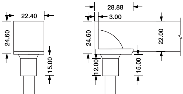
Bottom Entry Connector MJ-SF33-D5-B02SM MJ-SF33-D5-B03SFM
