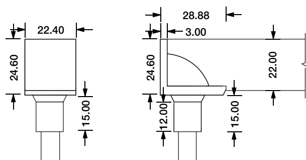
Bottom Entry Connector MJ-SF33-A-B01/02/03 MJ-SF33-A-B01SM MJ-SF33-A-B02SF MJ-SF33-A-B03SFM
