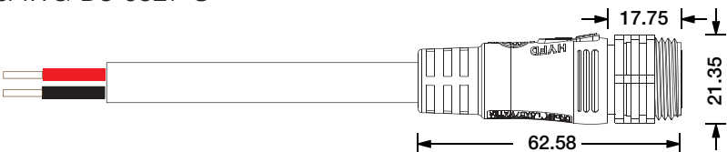
Male Connector SQ19-M-2C-15AWG-D8-0327-S
