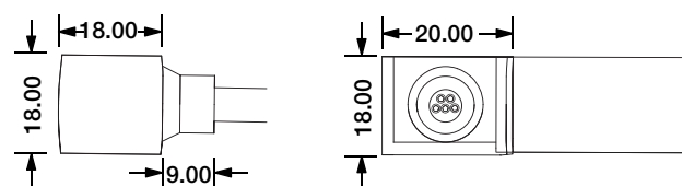
Side Entry Connector MJ-SF28-D5-S02SM MJ-SF28-D5-S03SFM
