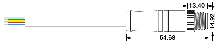
Male Connector M12-M-5C-18AWG+24AWG-D6-W-0327-S
