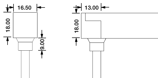
Bottom Entry Connector MJ-SF28-D5-B02SM MJ-SF28-D5-B03SFM
