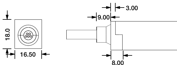
Direct Entry Connector MJ-SF28-D5-D02SM MJ-SF28-D5-D03SFM
