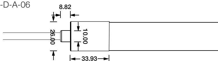
DIY Snap Front Connector DIY-SC-FR-SF24-D-A-06
