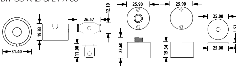
DIY Pendant Accessories Connector Kit DIY-SC-AAB-SF24-A-06
