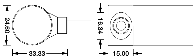
Side Entry Connector MJ-SF24-A-S01/02/03 MJ-SF24-A-S01SM MJ-SF24-A-S02SF MJ-SF24-A-S03SFM
