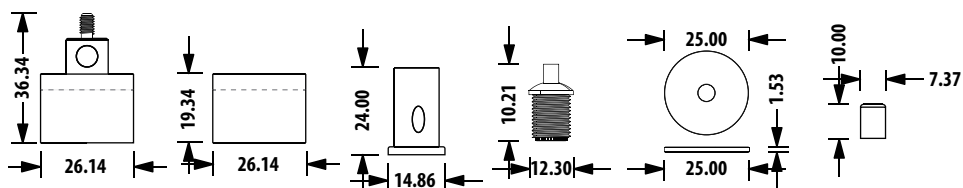
DIY Pendant Accessories Connector Kit DIY-SC-PA-SF24-A-06
