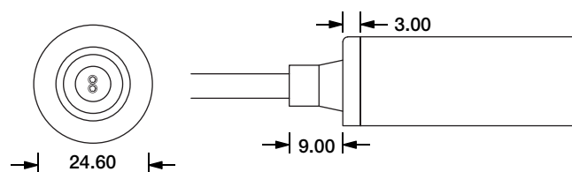
Direct Entry Connector MJ-SF24-A-D01/02/03 MJ-SF24-A-D01SM MJ-SF24-A-D02SF MJ-SF24-A-D03SFM
