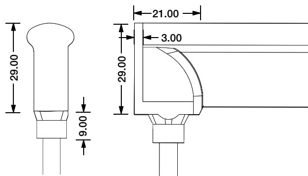
Bottom Entry Connector MJ-SF21-DW-B01/02/03 MJ-SF21-DW-B01SM MJ-SF21-DW-B02SF MJ-SF21-DW-B03SFM
