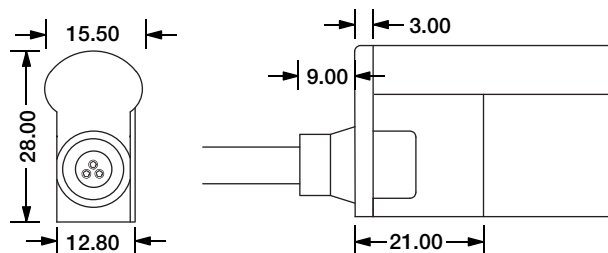
Direct Entry Connector MJ-SF21-DW-D01/02/03 MJ-SF21-DW-D01SM MJ-SF21-DW-D02SF MJ-SF21-DW-D03SFM
