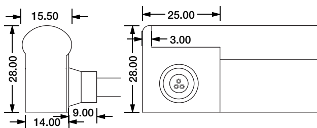
Side Entry Connector MJ-SF21-DW-S01/02/03 MJ-SF21-DW-S01SM MJ-SF21-DW-S02SF MJ-SF21-DW-S03SFM
