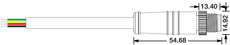
Male Connector M12-M-4C-20AWG-D6-W-0327-S
