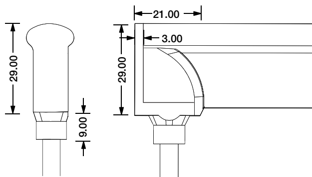
Bottom Entry Connector MJ-SF21-RGB-B01/02/03 MJ-SF21-RGB-B01SM MJ-SF21-RGB-B02SF MJ-SF21-RGB-B03SFM
