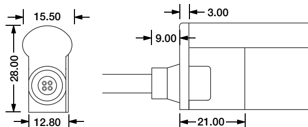
Direct Entry Connector MJ-SF21-RGB-D01/02/03 MJ-SF21-RGB-D01SM MJ-SF21-RGB-D02SF MJ-SF21-RGB-D03SFM
