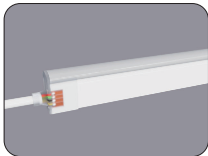
Direct Entry Connector MJ-SF21-RGB-D01/02/03 MJ-SF21-RGB-D01SM MJ-SF21-RGB-D02SF MJ-SF21-RGB-D03SFM
