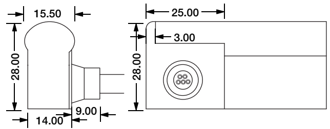
Side Entry Connector MJ-SF21-D5-S02SM MJ-SF21-D5-S03SFM
