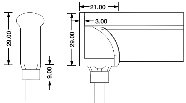
Bottom Entry Connector MJ-SF21-D5-B02SM MJ-SF21-D5-B03SFM
