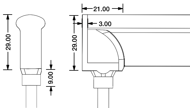
Bottom Entry Connector MJ-SF21-D3-B02SM MJ-SF21-D3-B03SFM
