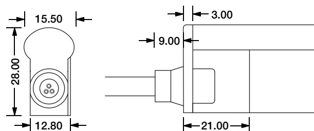
Direct Entry Connector MJ-SF21-D3-D02SM MJ-SF21-D3-D03SFM
