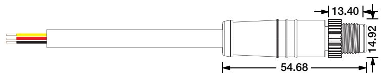
Male Connector M12-M-3C-20AWG-D6-W-0327-S
