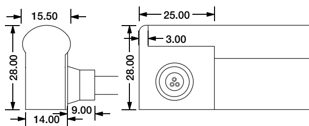
Side Entry Connector MJ-SF21-D3-S02SM MJ-SF21-D3-S02SFM
