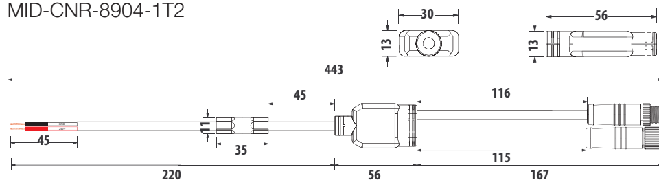
Middle Power Connector (1 to 2) MID-CNR-8904-1T2
