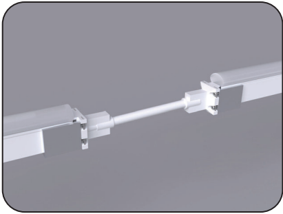
DIY Screw Extension Connector DIY-SC-EXT-15-A
