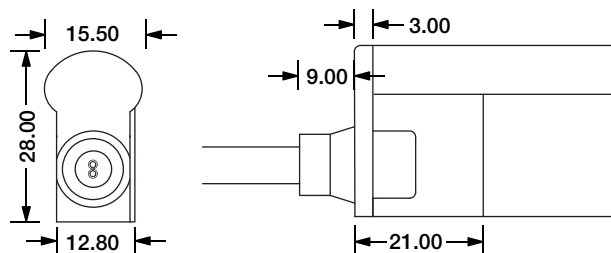
Direct Entry Connector MJ-SF21-A-D01/02/03 MJ-SF21-A-D01SM MJ-SF21-A-D02SF MJ-SF21-A-D03SFM
