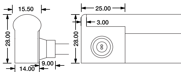
Side Entry Connector MJ-SF21-A-S01/02/03 MJ-SF21-A-S01SM MJ-SF21-A-S02SF MJ-SF21-A-S03SFM
