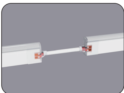
Jumper MJ-SF21-A-D-JC
