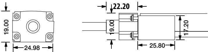
DIY Screw Connector DIY-SC-FR-16-D-01/02-DW
