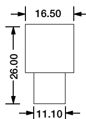
L Shape Entry Connector MJ-SF18-D3-L02SM MJ-SF18-D3-L03SFM
