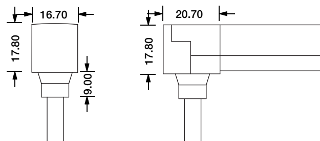
Bottom Entry Connector MJ-SF18-D3-B02SM MJ-SF18-D3-B03SFM
