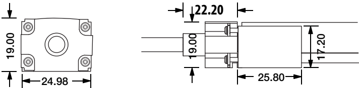
DIY Screw Connector DIY-SC-FR-16-D-01/02-D3
