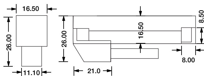
L Shape Entry Connector MJ-SF18-D3-L02SM MJ-SF18-D3-L03SFM
