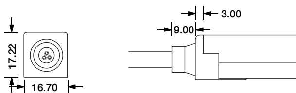
Direct Entry Connector MJ-SF18-D3-D02SM MJ-SF18-D3-D03SFM
