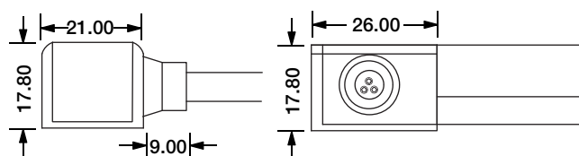
Side Entry Connector MJ-SF18-D3-S02SM MJ-SF18-D3-S03SFM
