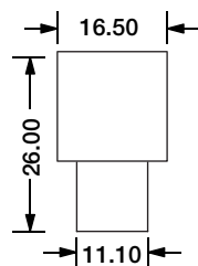
L Shape Entry Connector MJ-SF18-D3-L02SM MJ-SF18-D3-L03SFM
