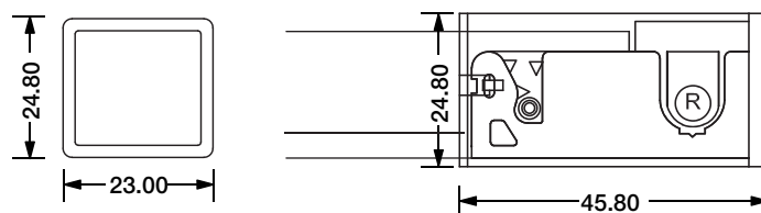
DIY Snap Extent Connector DIY-SN-EXT-16-D3
