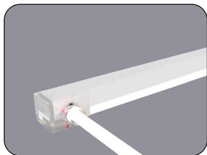
Side Entry Connector MJ-SF18-D3-S02SM MJ-SF18-D3-S03SFM
