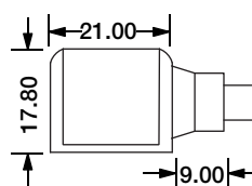
Side Entry Connector MJ-SF18-D3-S02SM MJ-SF18-D3-S03SFM
