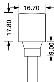
Bottom Entry Connector MJ-SF18-D3-B02SM MJ-SF18-D3-B03SFM
