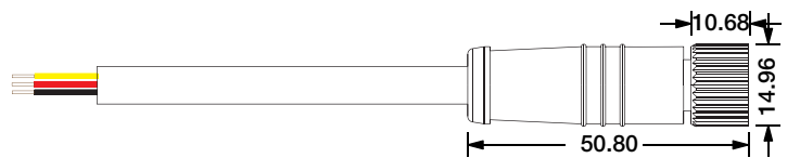
Female Connector M12-F-3C-20AWG-D6-W-0327-S
