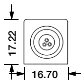
Direct Entry Connector MJ-SF18-D3-D02SM MJ-SF18-D3-D03SFM
