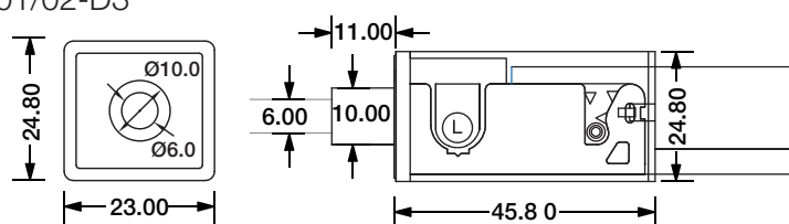
DIY Snap Connector DIY-SN-FR-16-D-01/02-D3
