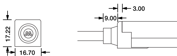
Direct Entry Connector MJ-SF18-D5-D02SM MJ-SF18-D5-D03SFM
