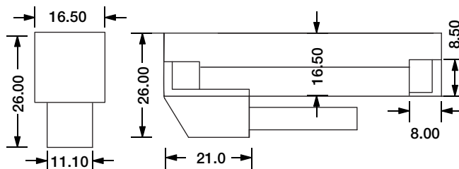
L Shape Entry Connector MJ-SF18-D5-L02SM MJ-SF18-D5-L03SFM
