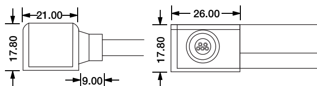
Side Entry Connector MJ-SF18-D5-S02SM MJ-SF18-D5-S03SFM
