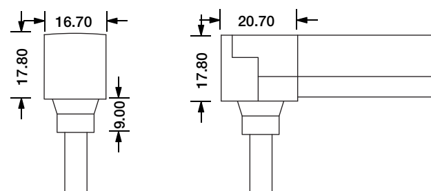
Bottom Entry Connector MJ-SF18-D5-B02SM MJ-SF18-D5-B03SFM
