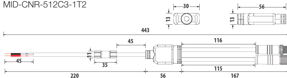
Middle Power Connector (1 to 2) MID-CNR-512C3-1T2
