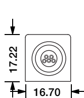
Direct Entry Connector MJ-SF18-D5-D02SM MJ-SF18-D5-D03SFM
