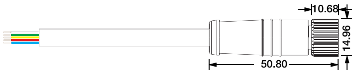
Female Connector M12-F-5C-18AWG+24AWG-D6-W-0327-S
