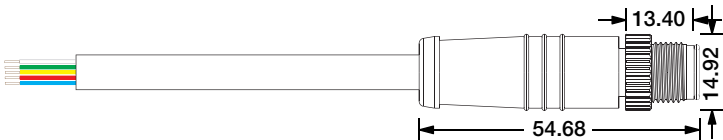
Male Connector M12-M-5C-18AWG+24AWG-D6-W-0327-S
