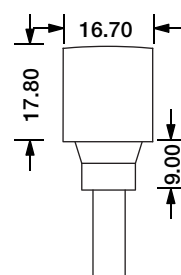
Bottom Entry Connector MJ-SF18-D5-B02SM MJ-SF18-D5-B03SFM
