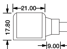
Side Entry Connector MJ-SF18-D5-S02SM MJ-SF18-D5-S03SFM
