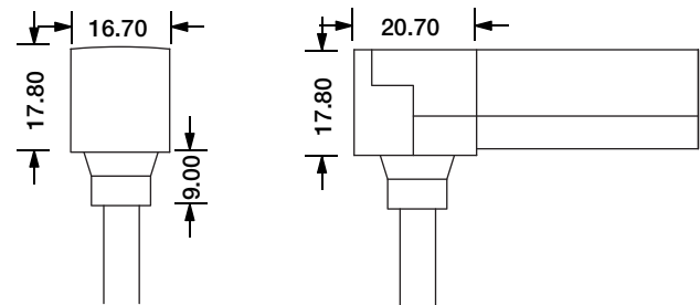
Bottom Entry Connector MJ-SF18-D5-B02SM MJ-SF18-D5-B03SFM
