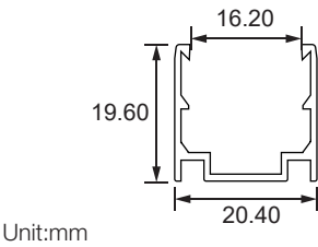
Dimension
