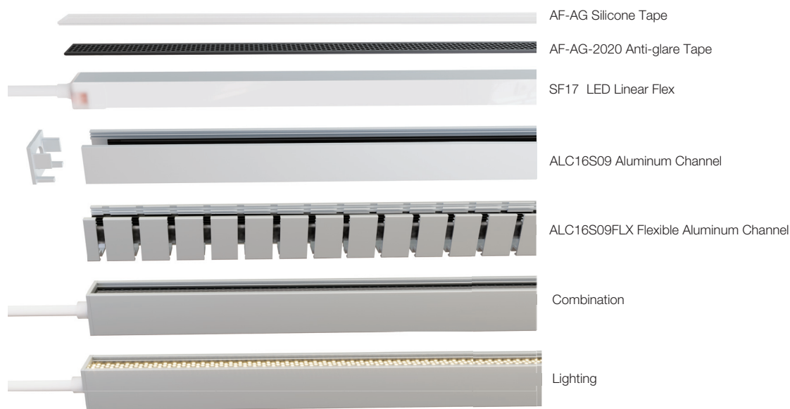
Surface Mounted
