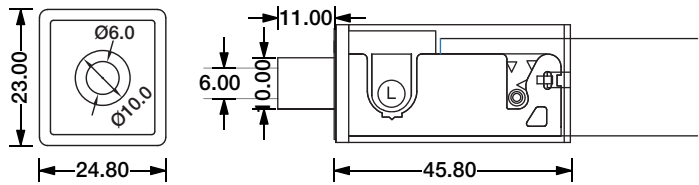
DIY Snap Connector DIY-SN-FR-17-D-01/02-D3
