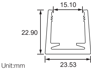
Dimension
