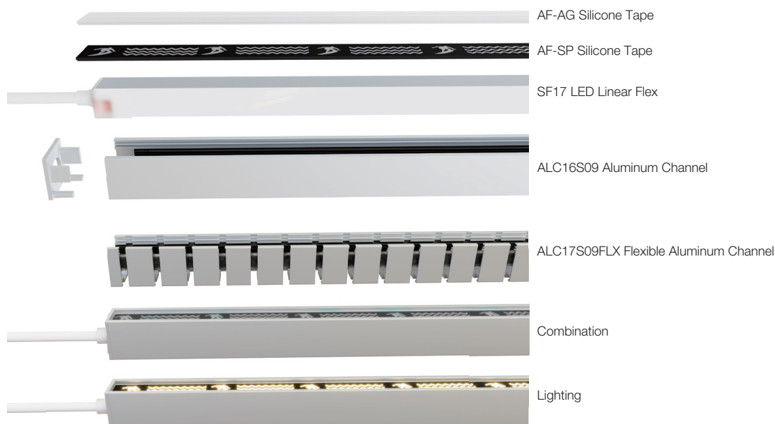
Surface Mounted
