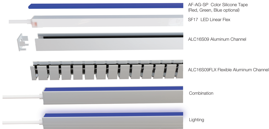
Surface Mounted
