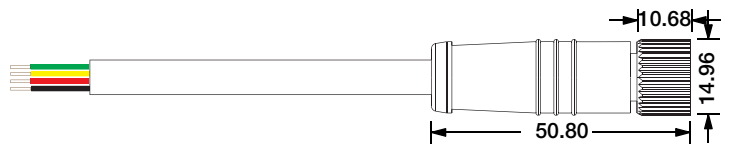
Female Connector M12-F-4C-20AWG-D6-W-0327-S
