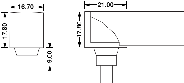
Bottom Entry Connector MJ-SF17-D3-B02SM MJ-SF17-D3-B03SFM
