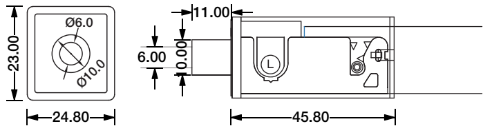
DIY Snap Connector DIY-SN-FR-17-D-01/02-D3
