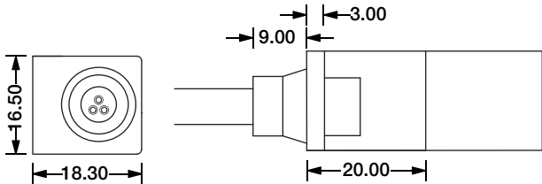
Direct Entry Connector MJ-SF17-D3-D02SM MJ-SF17-D3-D03SFM
