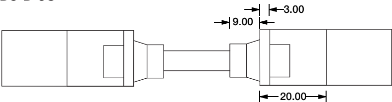
Jumper MJ-SF17-D3-D-JC
