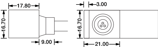
Side Entry Connector MJ-SF17-D3-S02SM MJ-SF17-D3-S03SFM
