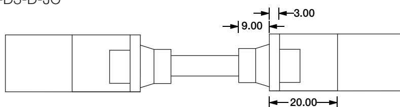
Jumper MJ-SF17-D3-D-JC
