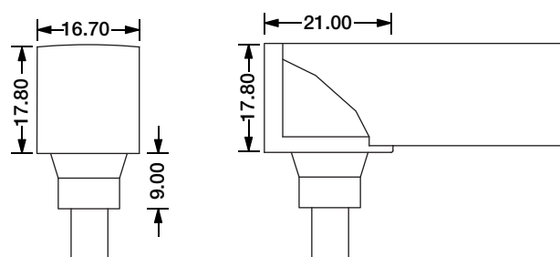
Bottom Entry Connector MJ-SF17-D3-B02SM MJ-SF17-D3-B03SFM
