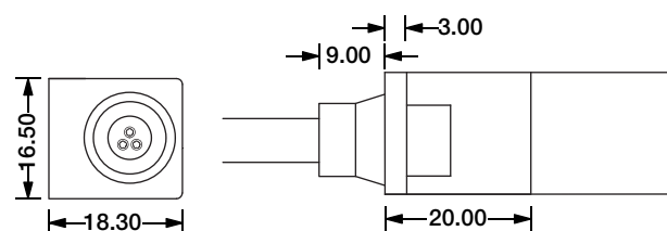
Direct Entry Connector MJ-SF17-D3-D02SM MJ-SF17-D3-D03SFM
