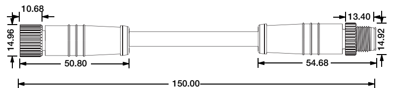
Positive Disconnected Connector Cable M12-EXT-SIG-5C-20AWG-D6-W-015
