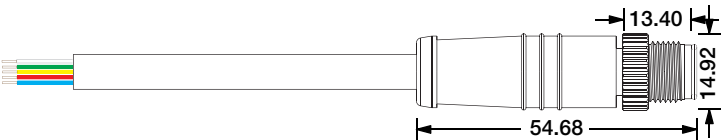
Male Connector M12-M-5C-20AWG-D6-W-0327-S
