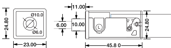
DIY Snap Connector DIY-SN-FR-16-D-01/02-RGB
