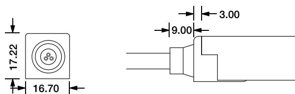
Direct Entry Connector MJ-SF16-D3-D02SM MJ-SF16-D3-D03SFM
