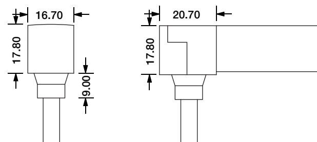
Bottom Entry Connector MJ-SF16-D3-B02SM MJ-SF16-D3-B03SFM
