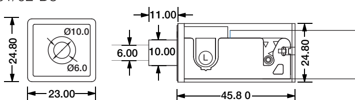
DIY Snap Connector DIY-SN-FR-16-D-01/02-D3
