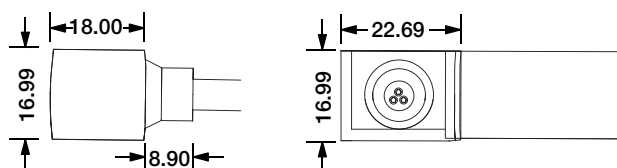
Side Entry Connector MJ-SF16-D3-S02SM MJ-SF16-D3-S03SFM
