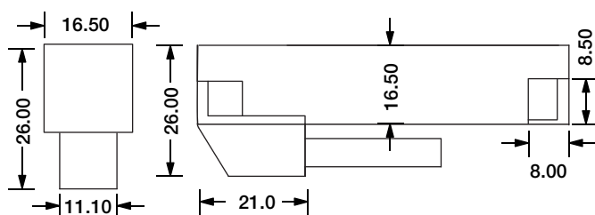
L Shape Entry Connector MJ-SF16-D3-L02SM MJ-SF16-D3-L02SFM
