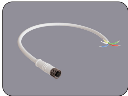
Female Connector M12-F-5C-18AWG+24AWG-D6-W-0327-S
