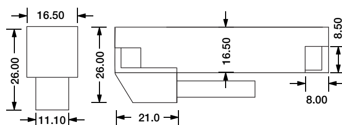
L Shape Entry Connector MJ-SF16-D5-L02SM MJ-SF16-D5-L02SFM
