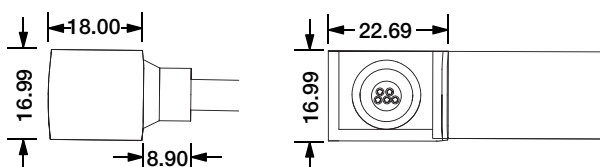
Side Entry Connector MJ-SF16-D5-S02SM MJ-SF16-D5-S03SFM
