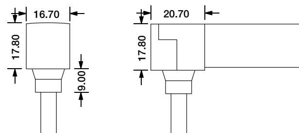
Bottom Entry Connector MJ-SF16-D5-B02SM MJ-SF16-D5-B03SFM
