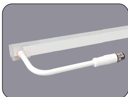
Side Entry Connector MJ-SF16-D5-S02SM MJ-SF16-D5-S03SFM
