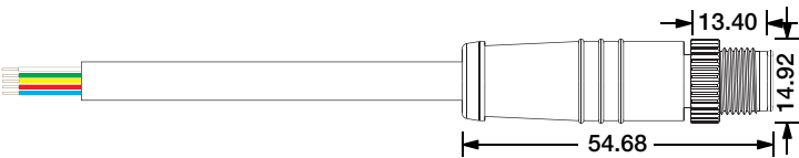
Male Connector M12-M-5C-18AWG+24AWG-D6-W-0327-S
