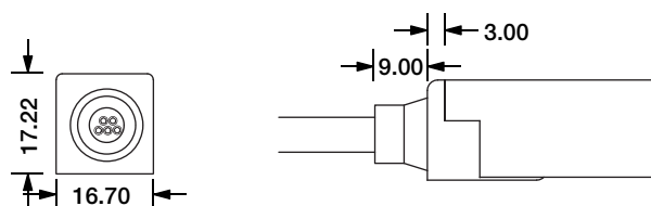
Direct Entry Connector MJ-SF16-D5-D02SM MJ-SF16-D5-D03SFM
