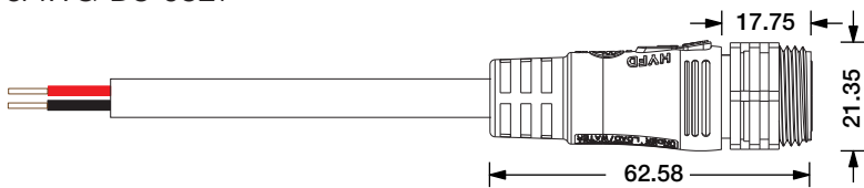
Male Connector SQ19-A-2P-M-15AWG-D8-0327
