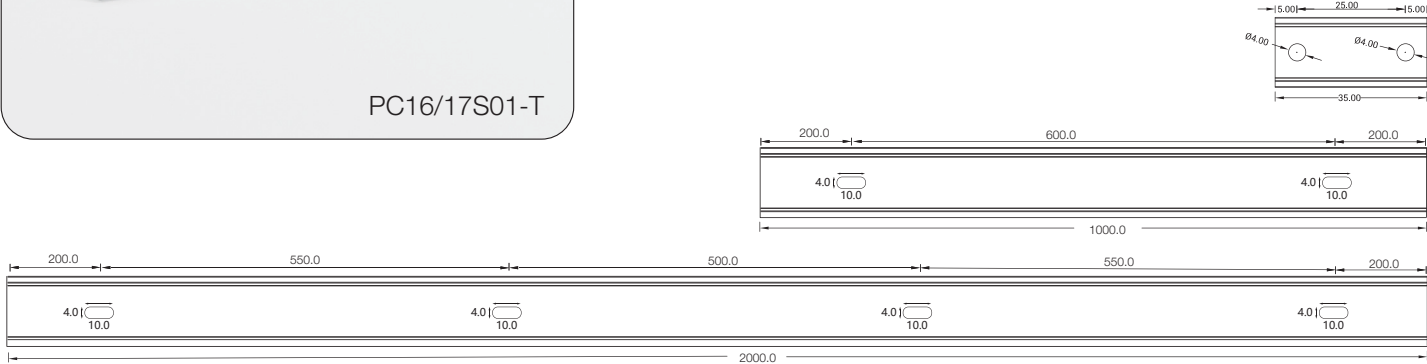
Surface Mounted
