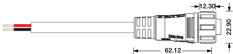
Female Connector SQ19-A-2P-F-15AWG-D8-032 7
