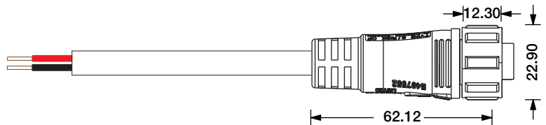
Female Connector SQ19-A-2P-F-15AWG-D8-032 7
