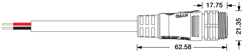
Male Connector SQ19-A-2P-M-15AWG-D8-0327
