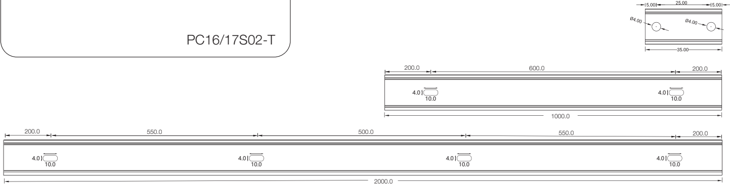
Surface Mounted
