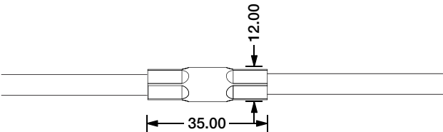
Waterproof Interrupter
